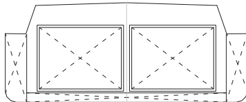
Type G Condition of cargo tank 2, Type of cargo tank 1 (also by flush-deck)
