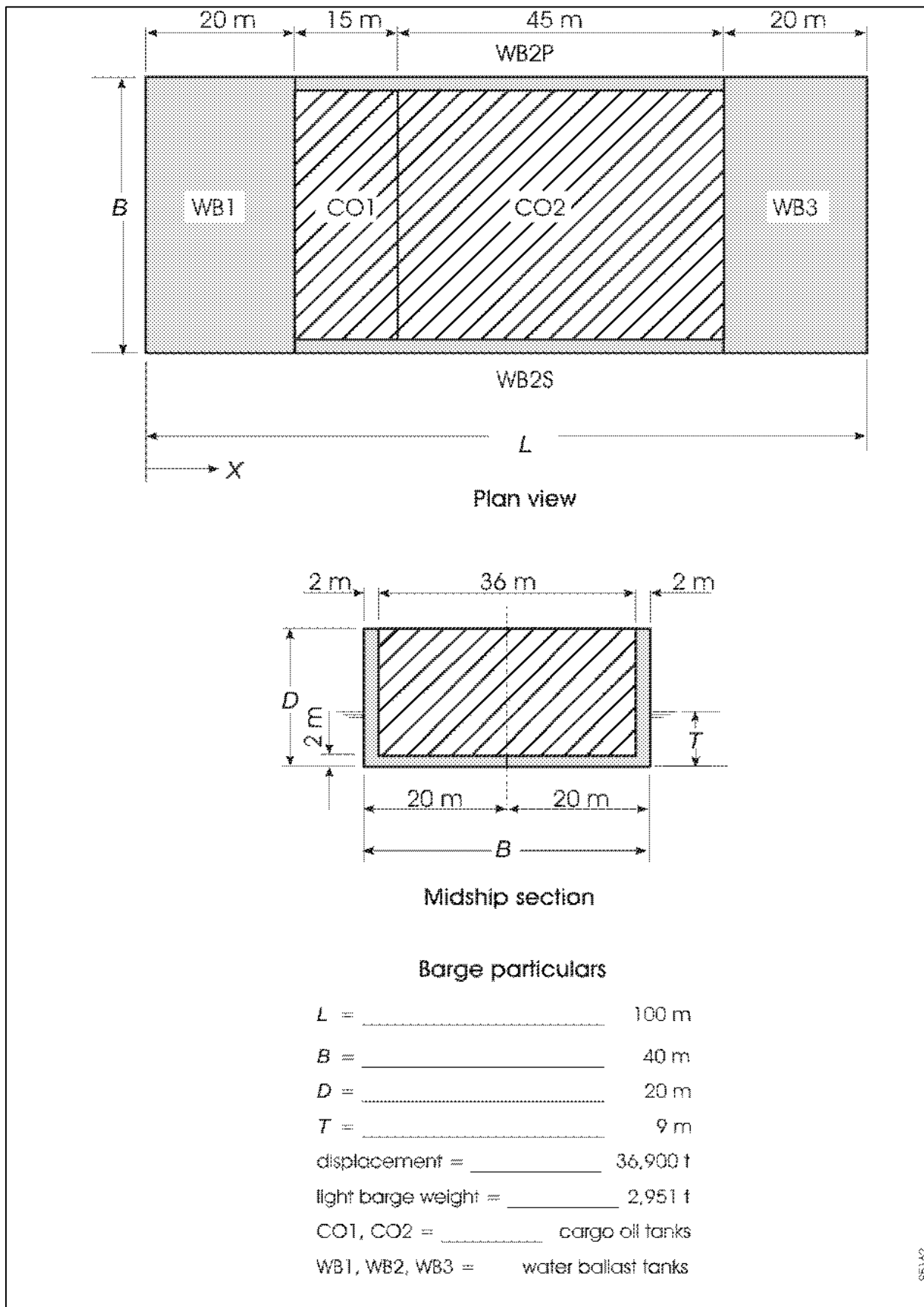
Figure A1 – Barge arrangement
