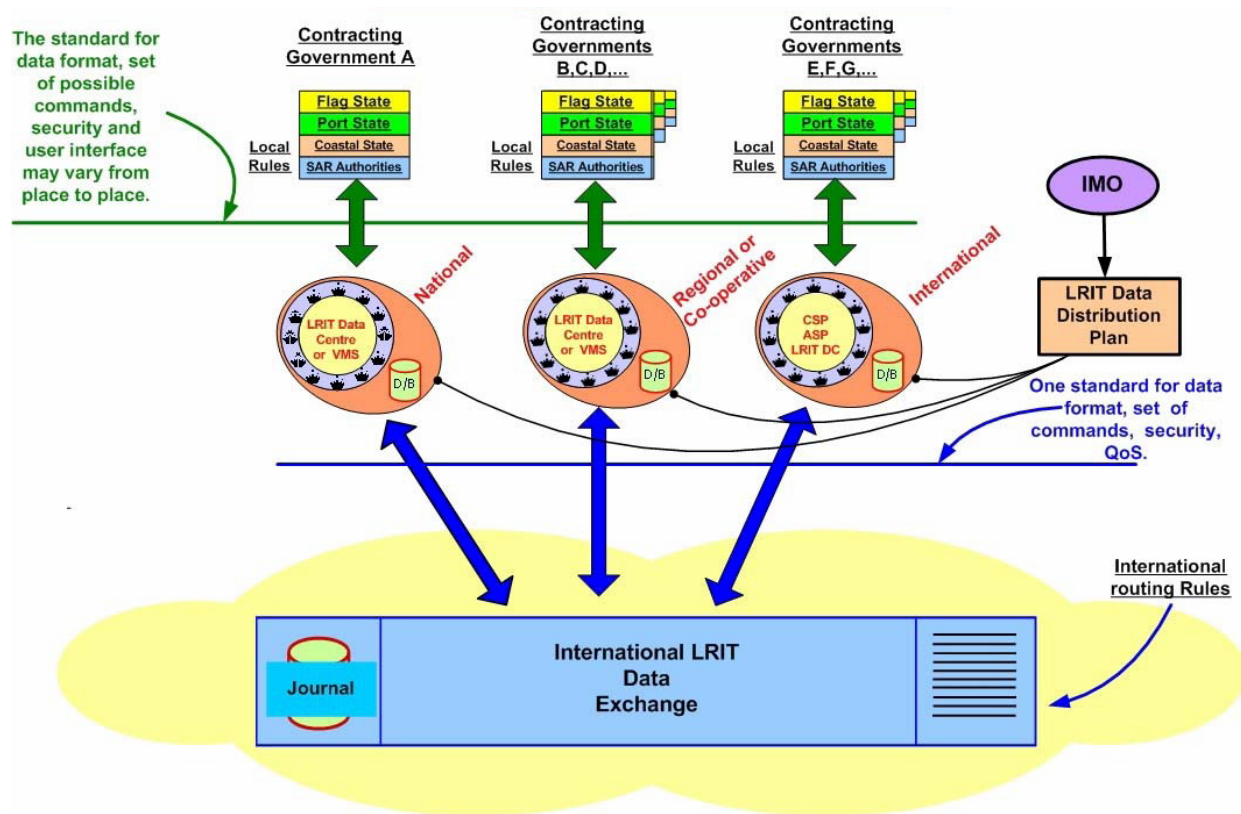
FIGURE 1 TYPICAL LRIT SYSTEM ARCHITECTURE
