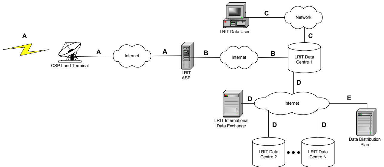
FIGURE 2 LRIT COMMUNICATIONS SEGMENTS
