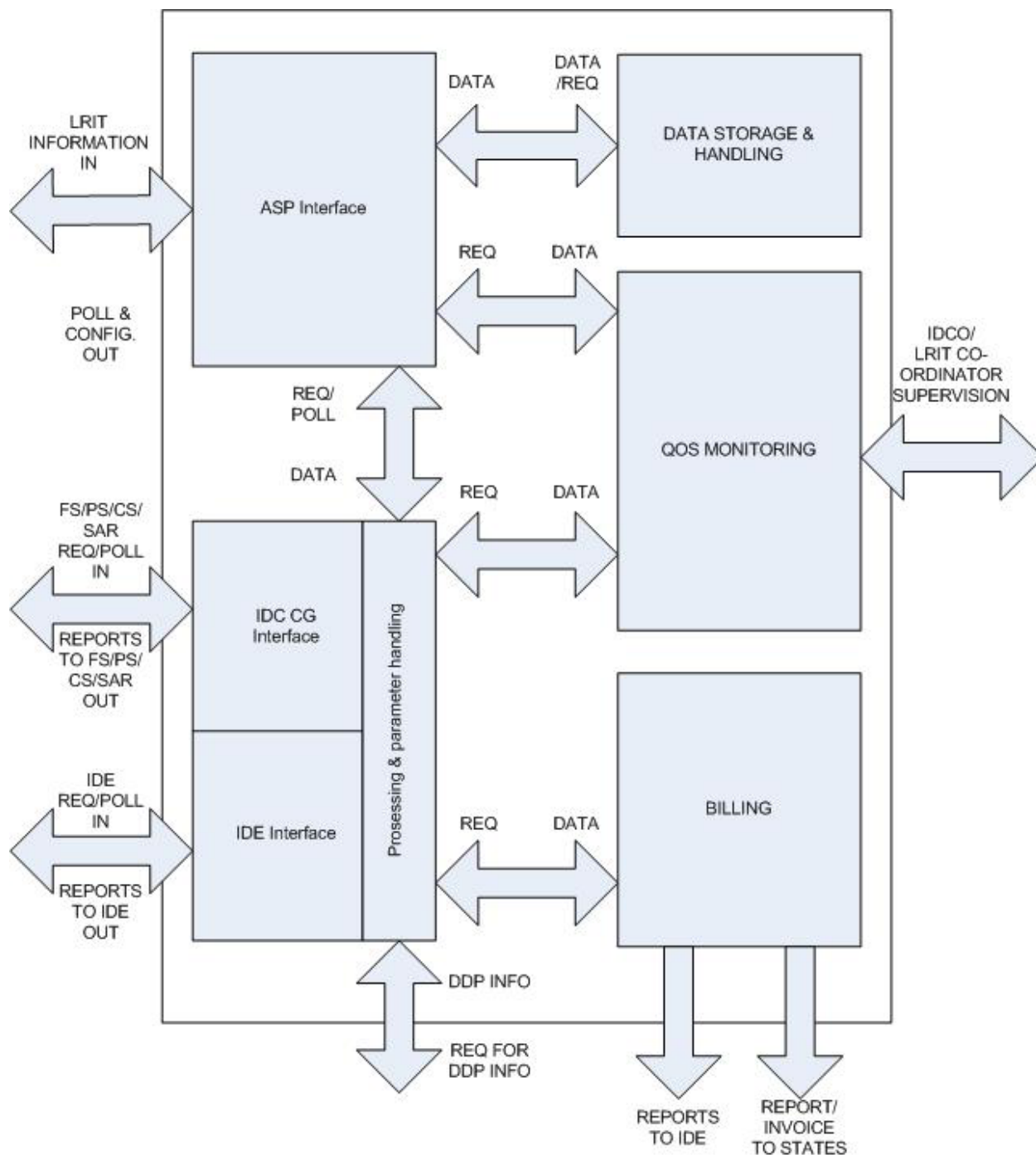
FIGURE 2 TOP LEVEL BLOCK SCHEMATIC DIAGRAM (1)
