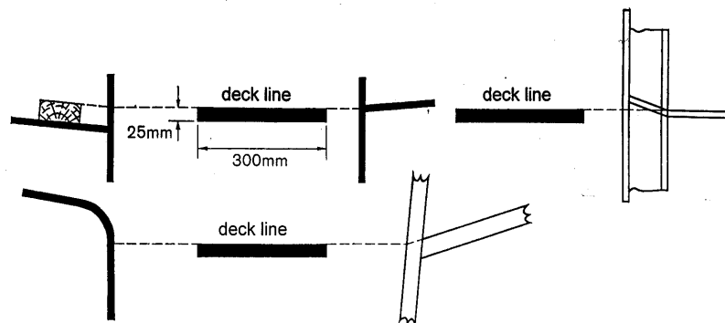
Figure 4.1 Deck line
