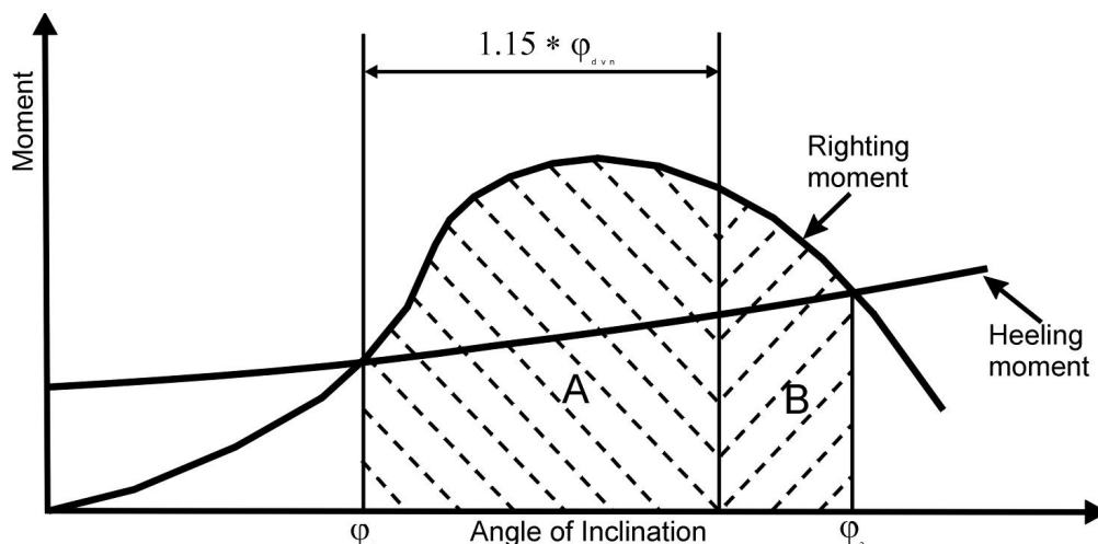
Figure 2.6-3 – Righting moment and heeling moment curves
